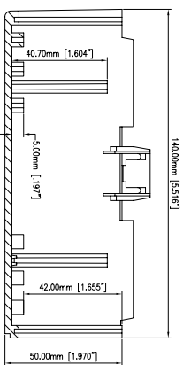
Section A-A High Case
