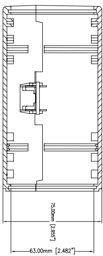
MEDIUM VERSION SIDE VIEW
