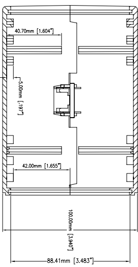
HIGH VERSION SIDE VIEW
