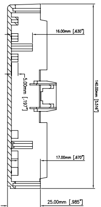
Section A-A Low Case
