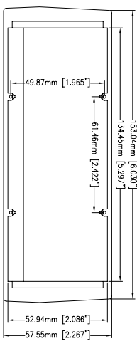
OPTIMAL SLOPE PANEL BACK VIEW (MEDIUM VERSION ONLY)
