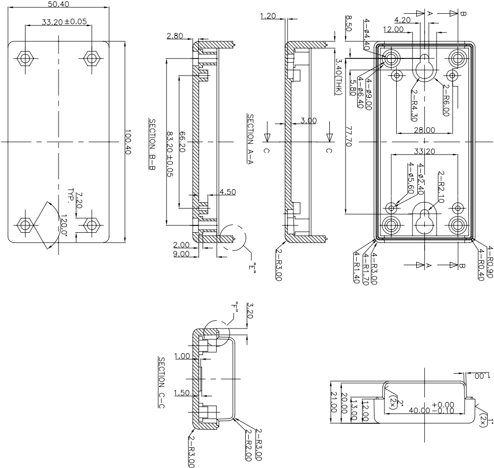
CASE BOTTOM SECTION VIEWS
